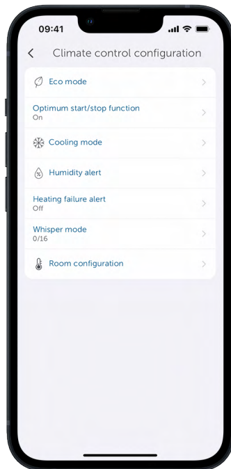
Abbildung 30: Screenshot Overview climate control configuration
