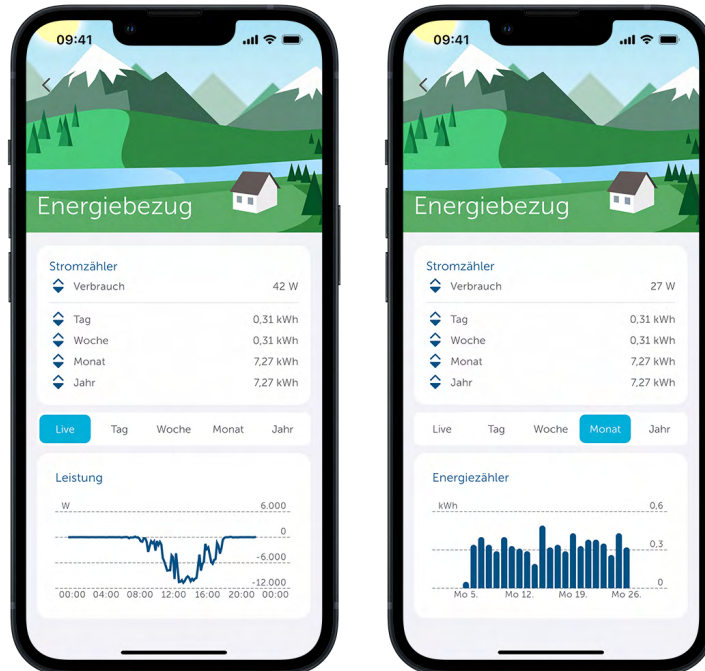
Abbildung 40: Detail page of the energy purchase
