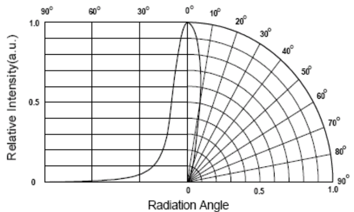
Radiation Characteristics
