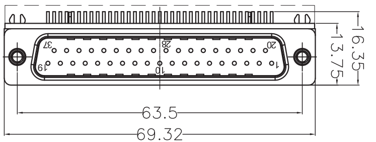
2X #4-40 JACKSCREW
