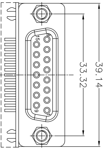
FEMALE 15P CONTACT D-SUB CONNECTOR
