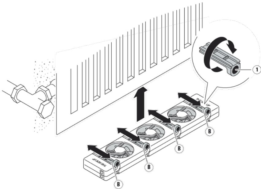
Fig. 7 - Attach the SpeedComfort (A) to a single plate radiator.
