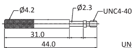
Long Screw
