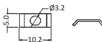
Washer
