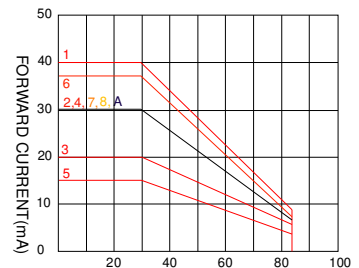
AMBIENT TEMPERATURE Ta(°C) FORWARD CURRENT VS. TEMPERATURE
