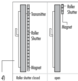
Positioning Roller Shutter Transmitter (side view)
