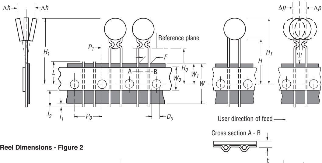
Taped Component Dimensions - Figure 1
