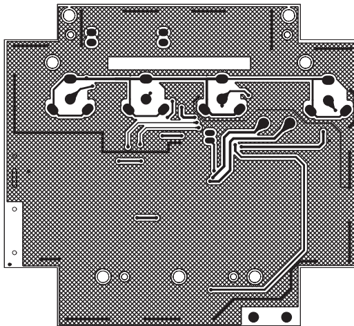
BOTTOM COPPER
