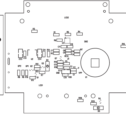
TOP SILKSCREEN
