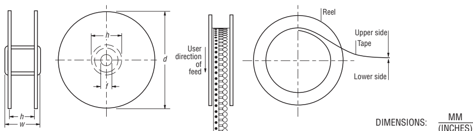
Reel Dimensions - Figure 2
