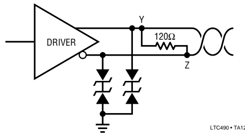
Figure 11. ESD Protection with TransZorbs®
