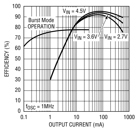
3-Cell to 5V Boost Efficiency
