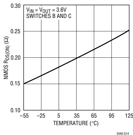
NMOS R DS(ON)
