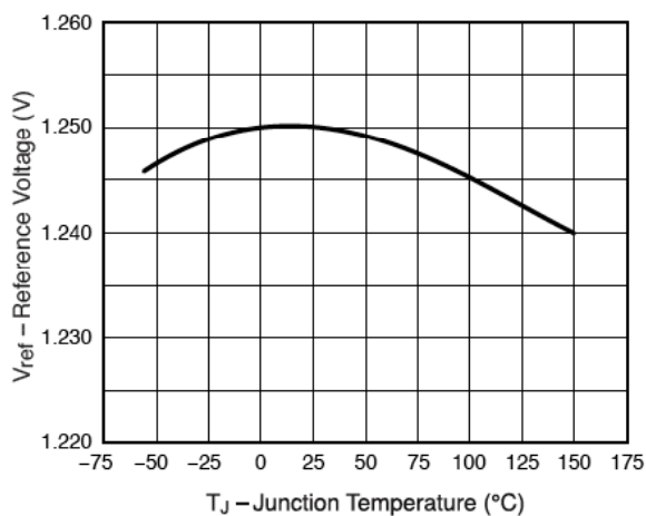
Figure 9. Temperature Stability
