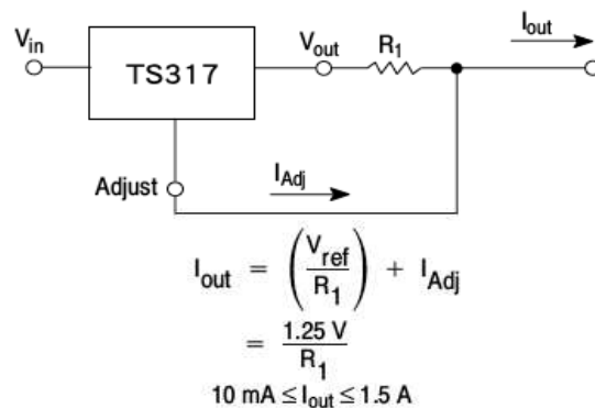
Figure 23. Current Regulator
