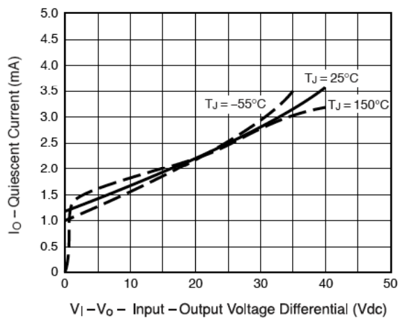
Figure 10. Minimum Operating Current
