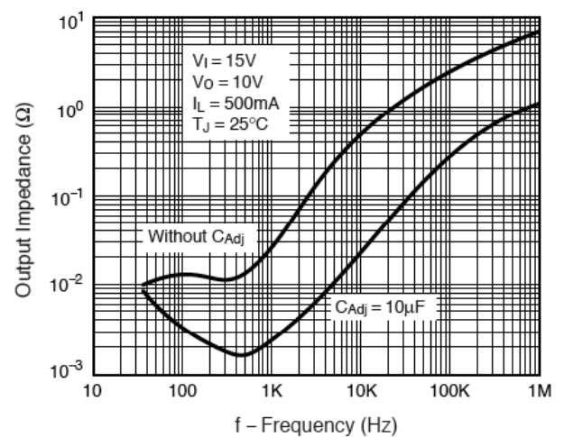
Figure 14. Output Impedance
