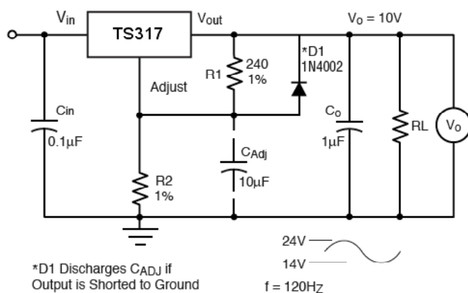
Figure 4. Ripple Rejection Test Circuit
