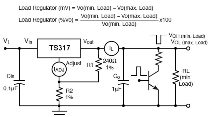
Figure 2. Load Regulation and \Delta I_{adj}/\text{Load} Test Circuit
