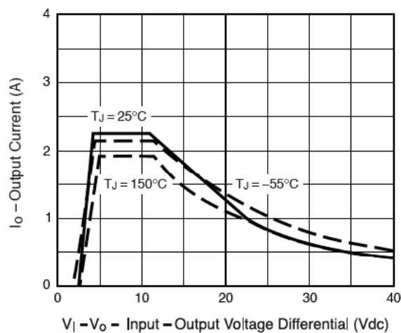
Figure 6. Current Limit
