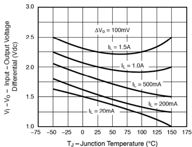
Figure 8. Dropout Voltage
