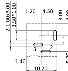
Pin Hole Layout (Jack Bottom View)
