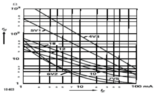
FIG.6- DYNAMIC RESISTANCE VS ZENER CURRENT
