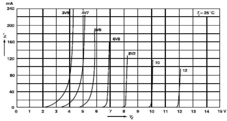
FIG.8- BREAKDOWN CHARACTERISTICS
