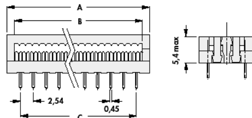
Forme DIL
